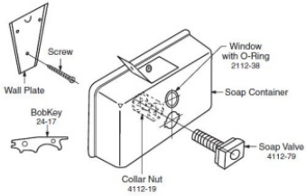
Bobrick B-2112 Parts Diagram
