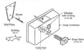
Bobrick B-2112 Parts Diagram
