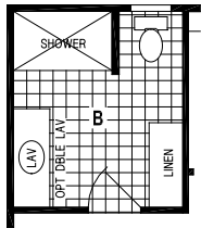
OPTION 60" SHOWER
