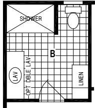
OPTION 60" SHOWER
