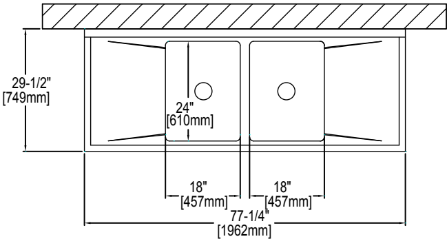
S/S SINKTOP & BACKSPLASH
