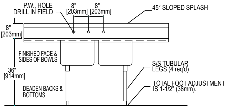
S/S SINKTOP & BACKSPLASH
